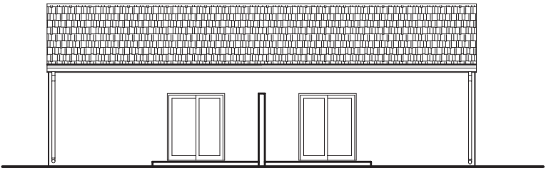
BACK ELEVATION
